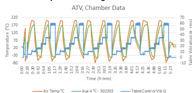
Figure 3. Levels of Vibration introduced during Repeated Cycles of Temperature and Rates of Temperature Changes
