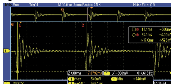
Figure 2. Shock Profile
